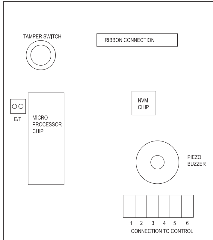
Figure 4. Keypad connections
